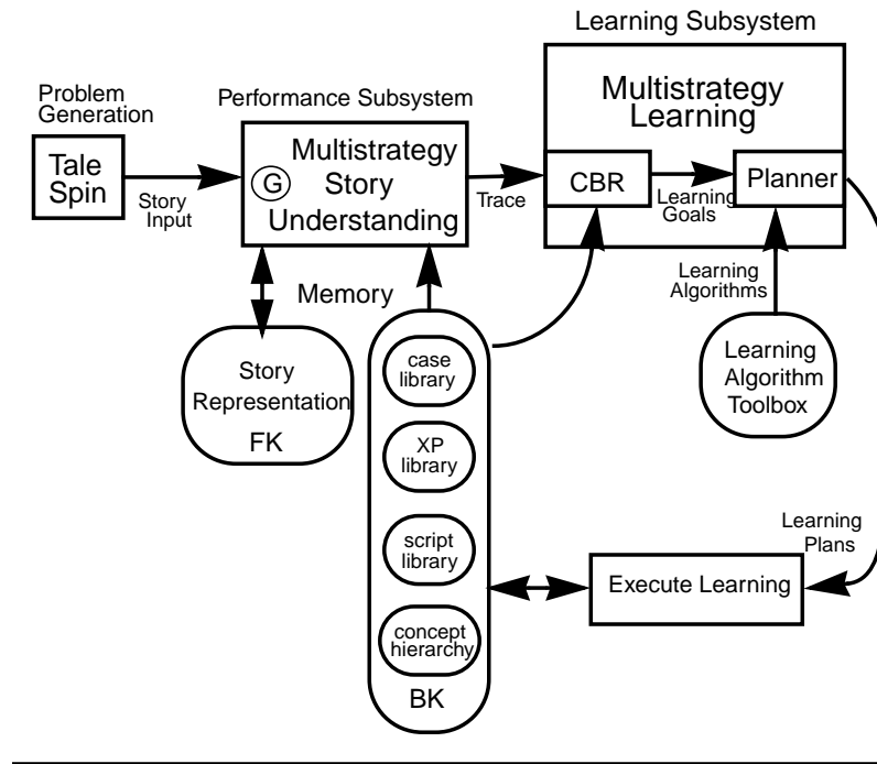
Fig. 6. Detailed Meta-AQUA system architecture
