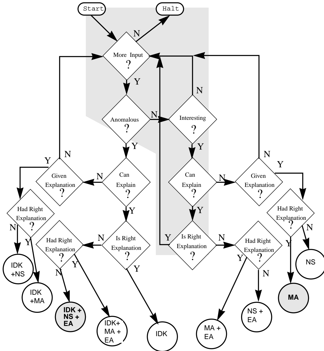
Fig. 24. Implemented space of reasoning faults
