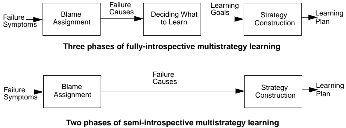
Fig. 25. Learning goal ablation
