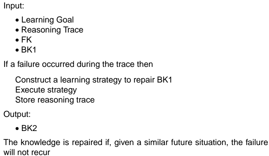
Fig. 11. Learning generation specification
