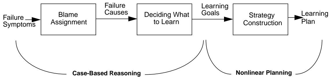
Fig. 1. Decomposition of the learning problem
