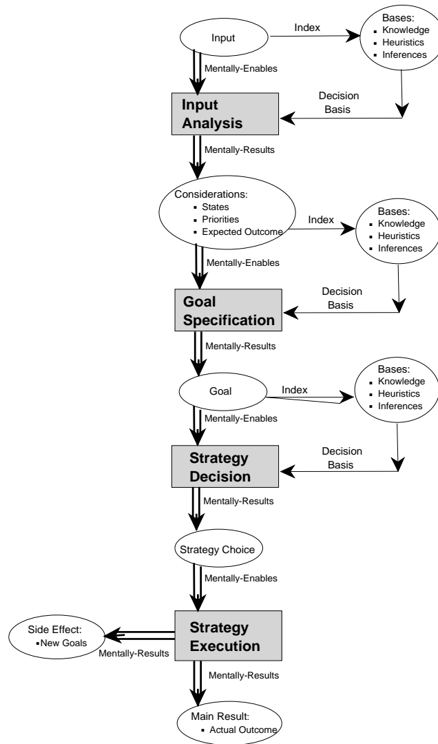
Fig. 9. Graph structure for Decide-Compute-Node
