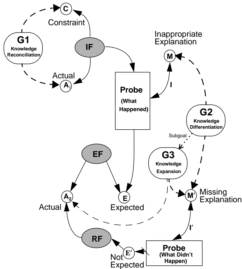
Fig. 16. Abstracted IMXP with learning goals
