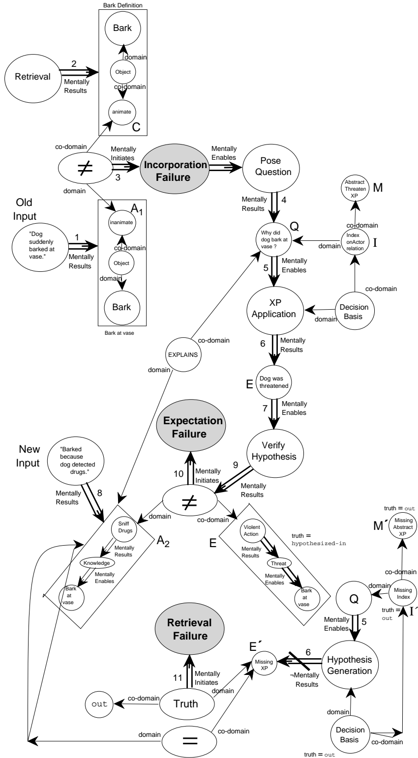
Fig. 15. Instantiated IMXP for mis-explanation
